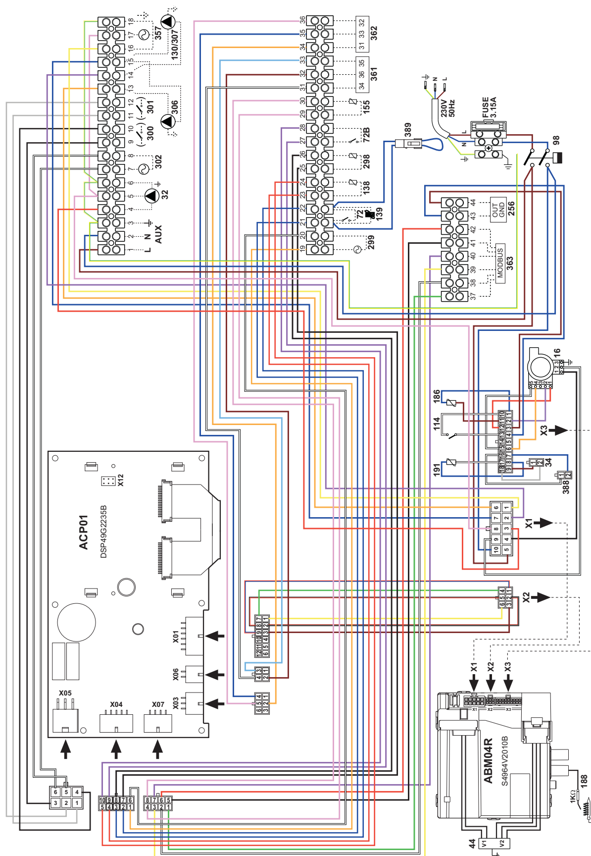
fig. 92- Wiring diagram - models TORO W 99, TORO W 120 and TORO W 150
