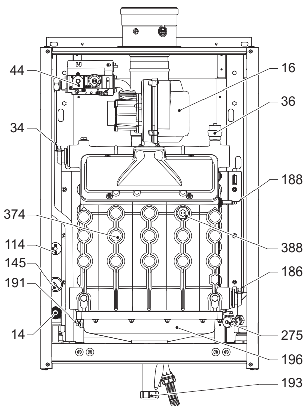
fig. 83- Vista general mod. TORO W 150
