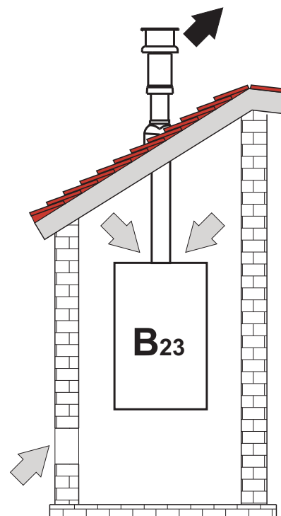
fig. 58- Connection examples (⇐=Air / ⇨=Fumes)
