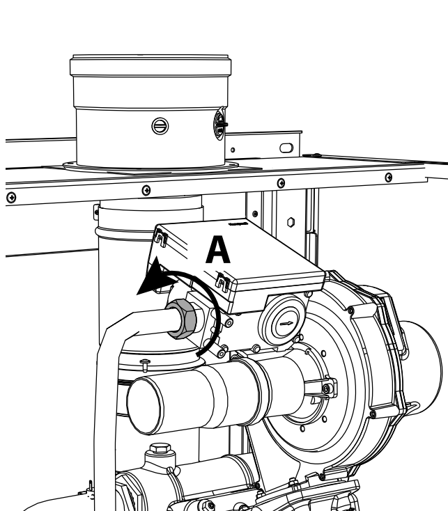
fig. 61- Models W 60 and W 80
