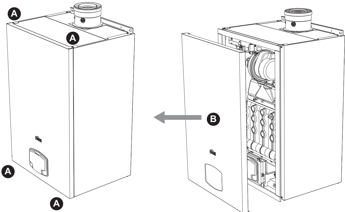
fig. 76- Front panel opening
