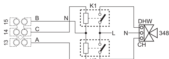
fig. 89- Connection of the 3-way valve with 3 wires
